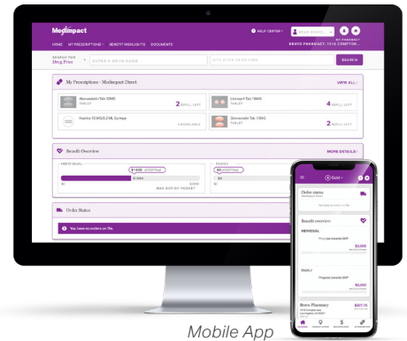
Mobile App
